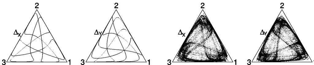
FIG. 2. Limit cycle (left, \epsilon_Y = 0.025 ) and chaotic attractor (right, \epsilon_Y = -0.365 ), with \epsilon_X = 0.5 , \alpha_X = \alpha_Y = 0.01 , and \beta_X = \beta_Y .
