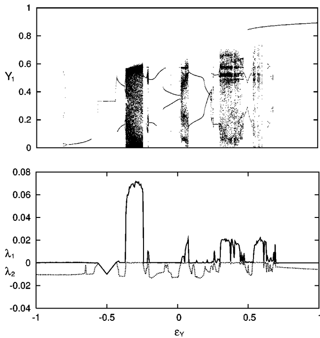
FIG. 3. Bifurcation diagram (top) of dissipative (learning with memory loss) dynamics projected onto coordinate y_1 from the Poincaré section hyperplane ( \dot{u}_1=0 , \dot{v}_1>0 ) and the largest two Lyapunov exponents \lambda_1 and \lambda_2 (bottom) as functions of \epsilon_Y \in [-1, 1] . Here with \epsilon_X=0.5 , \alpha_X=\alpha_Y=0.01 , and \beta_X=\beta_Y . Simulations show that \lambda_3 and \lambda_4 are always negative.
