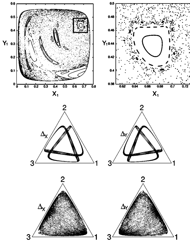
FIG. 1. Quasiperiodic tori and chaos: \epsilon_X = -\epsilon_Y = 0.5 , \alpha_X = \alpha_Y = 0 , and \beta_X = \beta_Y . We give a Poincaré section (top) on the hyperplane defined by \dot{u}_1 = 0 and \dot{v}_1 > 0 ; that is, in the (\mathbf{x}, \mathbf{y}) space: (3 + \epsilon_X)y_1 + (3 - \epsilon_X)y_2 - 2 = 0 and (3 + \epsilon_Y)x_1 + (3 - \epsilon_Y)x_2 - 2 < 0 . There are 23 randomly selected initial conditions with energies H = -1/3(u_1 + u_2 + v_1 + v_2) + \ln(1 + e^{u_1} + e^{u_2}) + \ln(1 + e^{v_1} + e^{v_2}) = 2.941\,693 , whose surface forms the outer border of H \leq 2.941\,693 . (Bottom rows): Representative trajectories, simulated with a fourth-order symplectic integrator [16], starting from initial conditions within the Poincaré section. The upper simplices show a torus in the section's upper right corner; see the enlarged section at the upper right. The initial condition is (\mathbf{x}, \mathbf{y}) = (0.3, 0.054\,196, 0.645\,804, 0.1, 0.2, 0.7) . The lower simplices are an example of a chaotic trajectory passing through the regions in the section that are a scatter of dots; the initial condition is (\mathbf{x}, \mathbf{y}) = (0.05, 0.35, 0.6, 0.1, 0.2, 0.7) .
